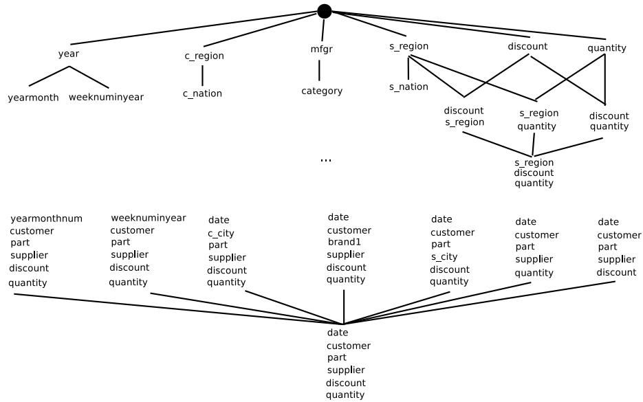
Fig. 1. Illustration of data cube lattice of SSB
